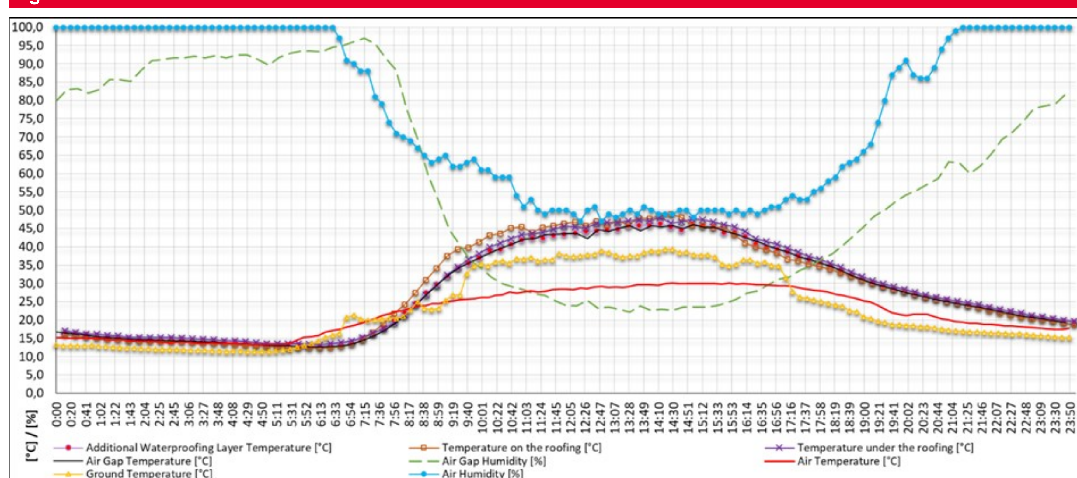
Figure 7. GRAPH OF THE COURSE OF TEMPERATURES AND HUMIDITY IN CRITICAL NORM DAY 21 ST AUGUST
